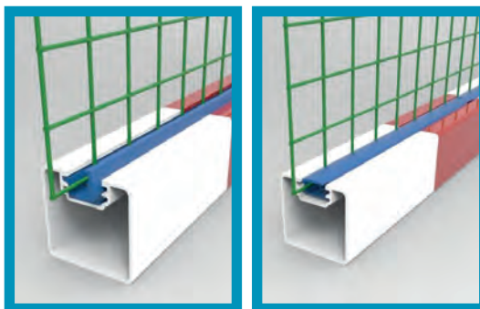
Integrated net hook system
