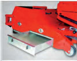
The vibrating screen separates dirt from the infill and spreads the infill on the artificial turf again at the same time
